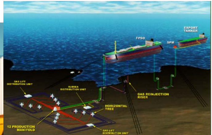
(Above) Kuito FPSO as it is operational offshore Angola for Chevron in 383 meters water depth: Floating, Producing, Storing, Offloading oil and using waterinjection to boost production.
